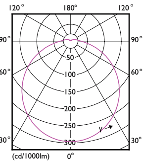
Light Distribution Diagram - UFO LEDBulb 15W E27 6500K 230V 1CT/6
